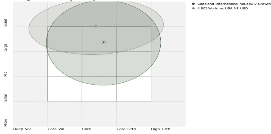
Holdings-Based Style Map
