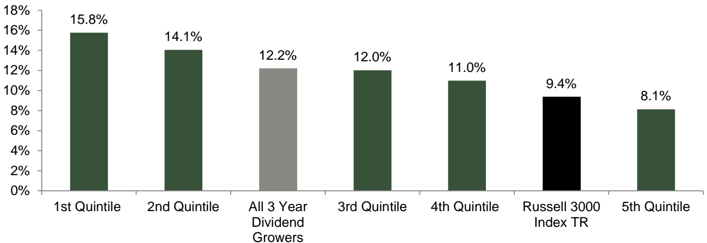
Output of Multi-Factor Model From 12/31/1989 to 12/31/2018
